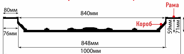
KP100-57 (1000x1000x71) рама: 1000x1000x12 короб: 848x848x59
