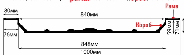
KP100-58 (1000x1000x71) рама: 1000x1000x12 короб: 848x848x59
