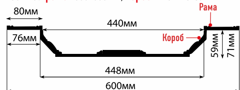
KS61-18D рама: 600x600x12, короб: 448x448x59
