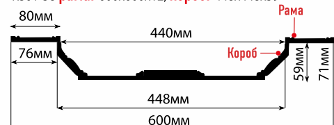
KS61-58 рама: 600x600x12, короб: 448x448x59
