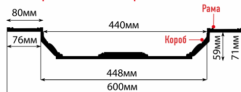
KS61-57 рама: 600x600x12, короб: 448x448x59
