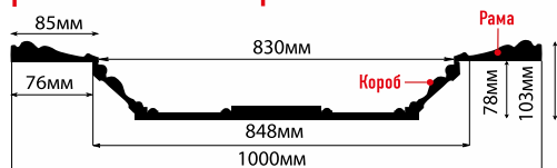
KP100-7D (1000x1000x103) рама: 1000x1000x25 короб: 848x848x78
