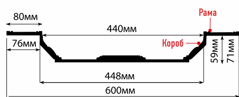
KS61-19D рама: 600x600x12, короб: 448x448x59
