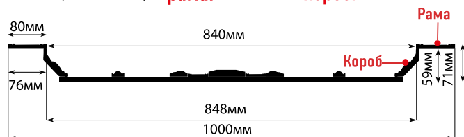
KP100-56 (1000x1000x71) рама: 1000x1000x12 короб: 848x848x59
